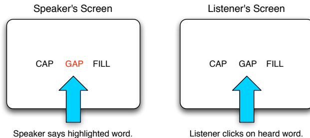
Figure 1: Experimental paradigm.
